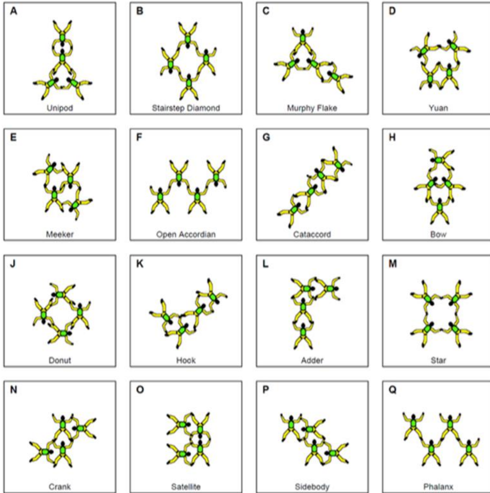
Attachement 1: Randoms
